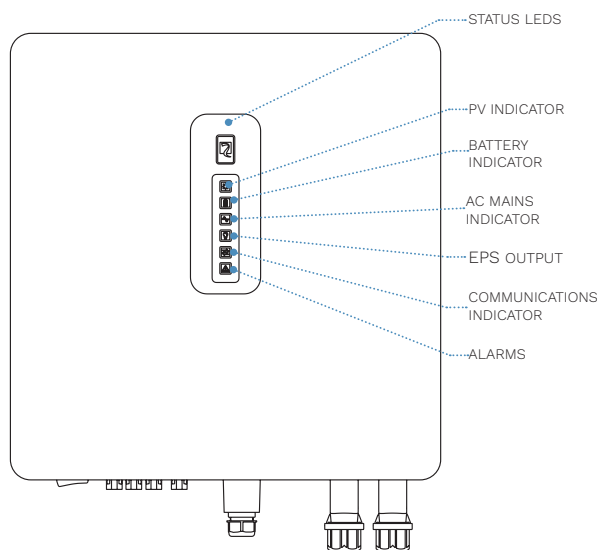
RS Hybrid three-phase 10 kW (front view)
